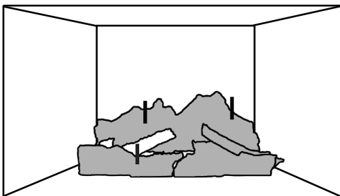
E. Place the lower left crossover log (W135-0698) in the notch of the left middle log.
